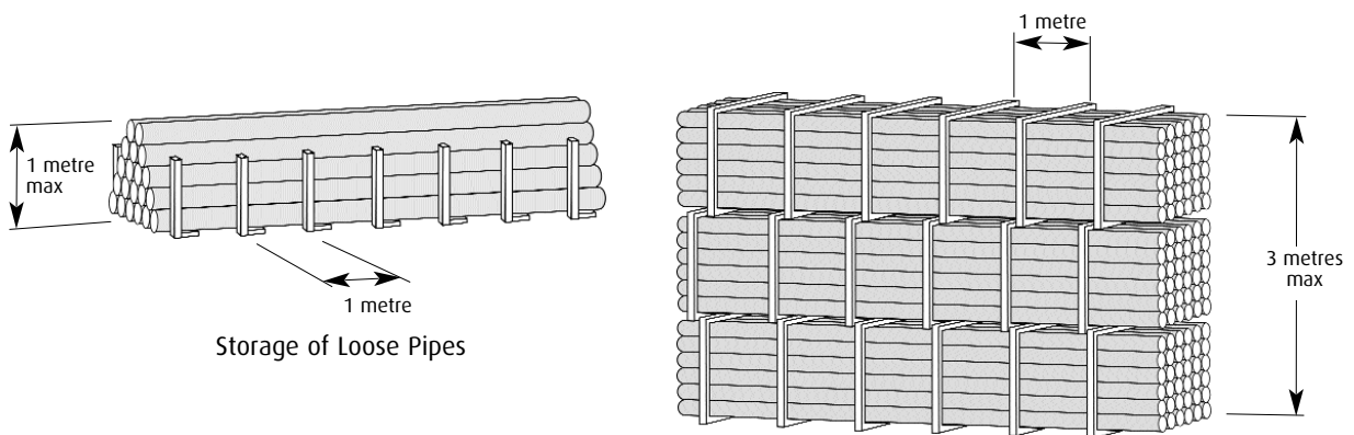
Storage of Bundled Pipes
